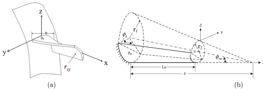
Figure 1: (a) Pretwisted turbo-machinery blade (b) Conical shell model.
