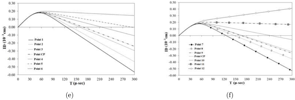
Figure 10: Effect of location of impact on contact force ( F_c ), deflection/thickness ( D/t ) and impactor's displacement (ID) with respect to time (T) at \psi=0^\circ, 45^\circ for Stainless Steel Nickel functionally graded conical shells considering time step ( \Delta t )= 1.0 \mu -sec, N=1 , t=0.002 m, VOI=3 m/s, Lo/s=0.7 , \phi_o=45^\circ , \phi_{ve}=20^\circ .
